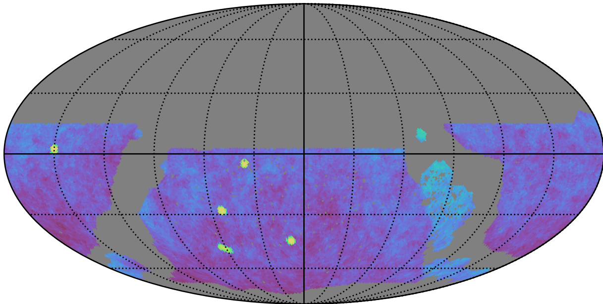
noroll_v3.4_10yrs gri WFD: Fraction of visits in pairs (10-60 min)
