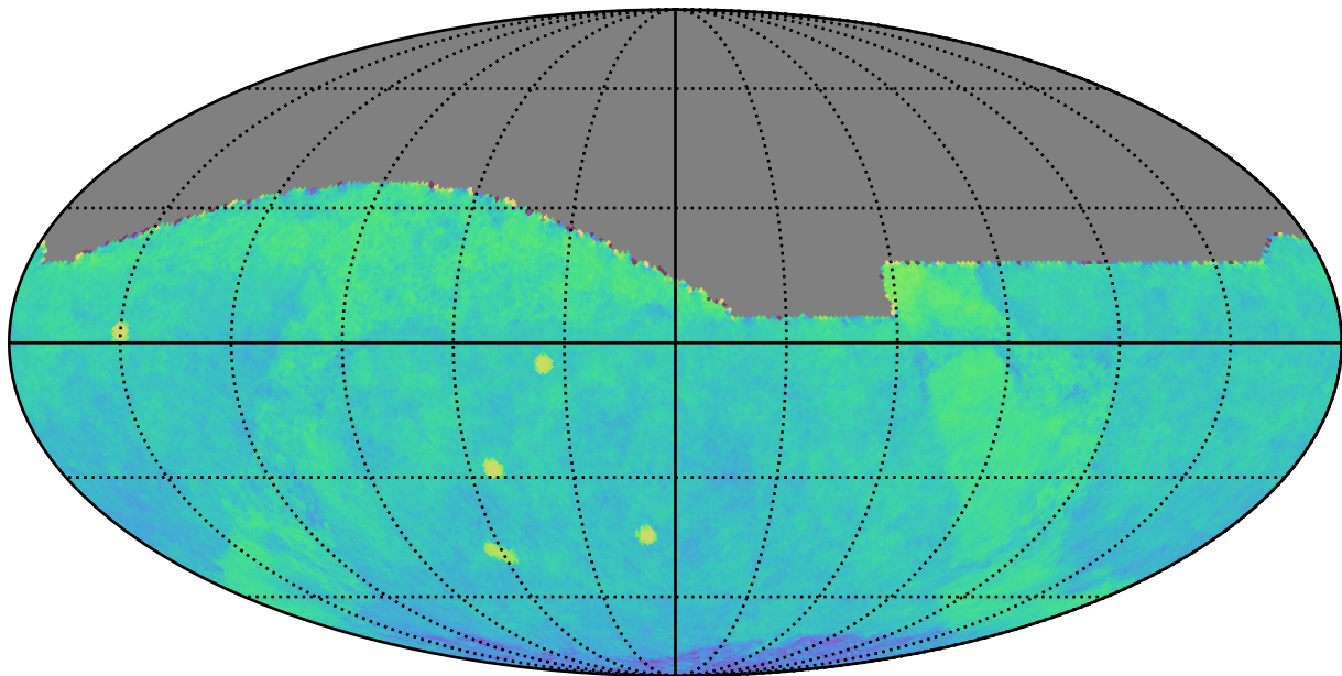
noroll_v3.4_10yrs gri All sky: Fraction of visits in pairs (10-60 min)
