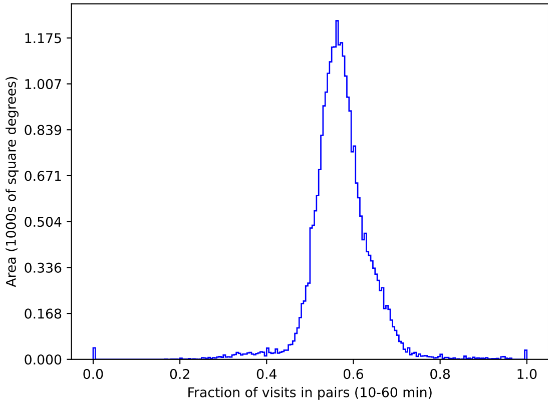
noroll_v3.4_10yrs gri All sky: Fraction of visits in pairs (10-60 min)
