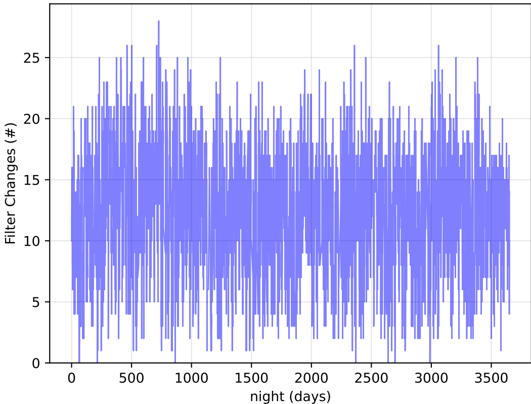
noroll_v3.4_10yrs Per Night: Filter Changes
