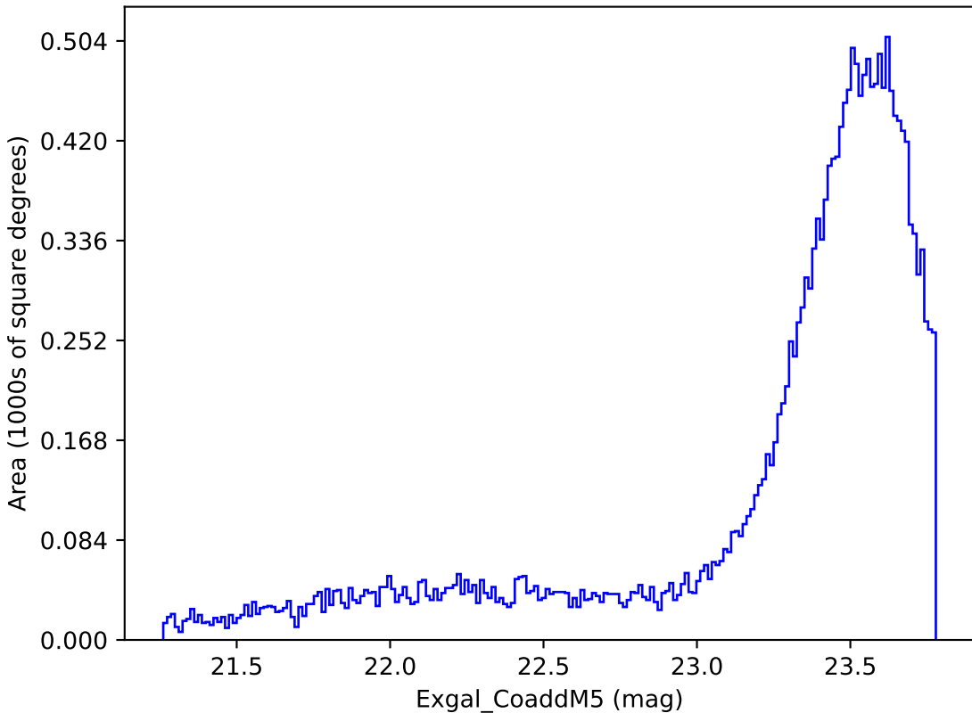
noroll_v3.4_10yrs Yr 3-4 y band: Exgal_CoaddM5
