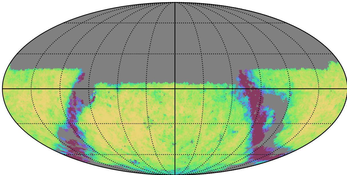
noroll_v3.4_10yrs Yr 3-4 u band: Exgal_CoaddM5
