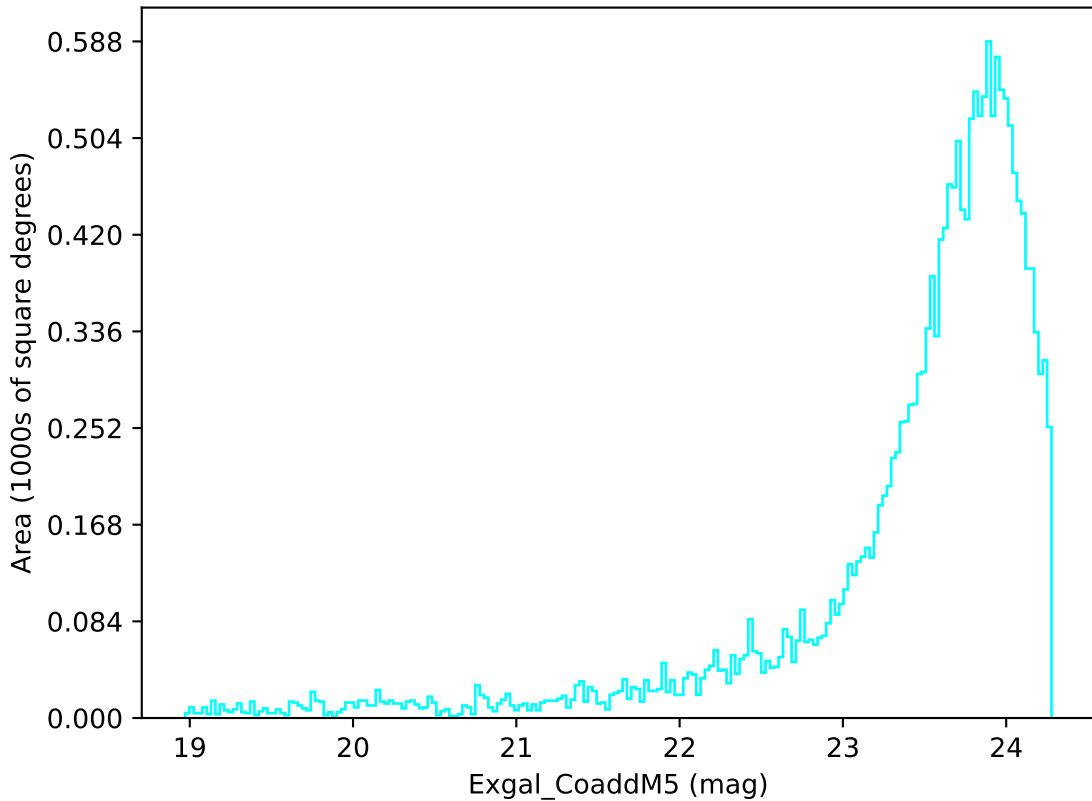
noroll_v3.4_10yrs Yr 3-4 u band: Exgal_CoaddM5
