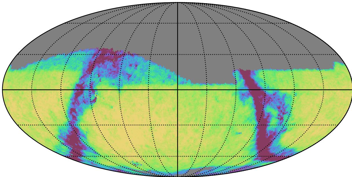
noroll_v3.4_10yrs Yr 3-4 r band: Exgal_CoaddM5
