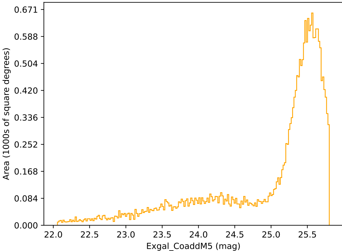
noroll_v3.4_10yrs Yr 3-4 r band: Exgal_CoaddM5
