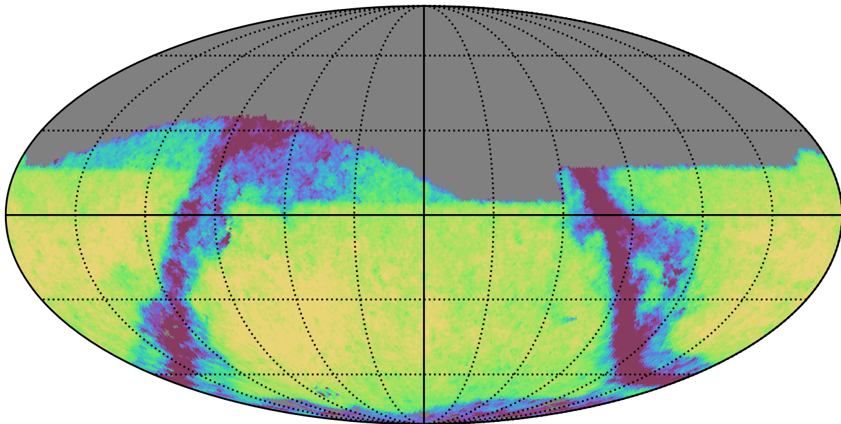
noroll_v3.4_10yrs Yr 3-4 i band: Exgal_CoaddM5
