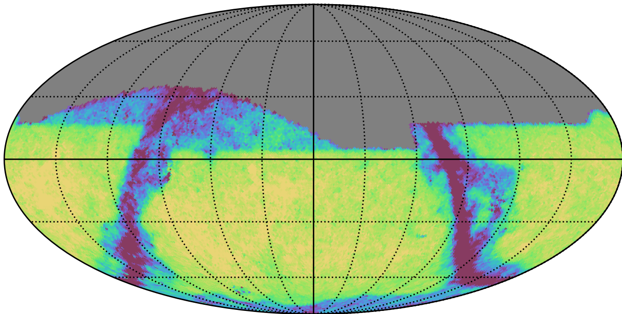
noroll_v3.4_10yrs Yr 1 z band: Exgal_CoaddM5
