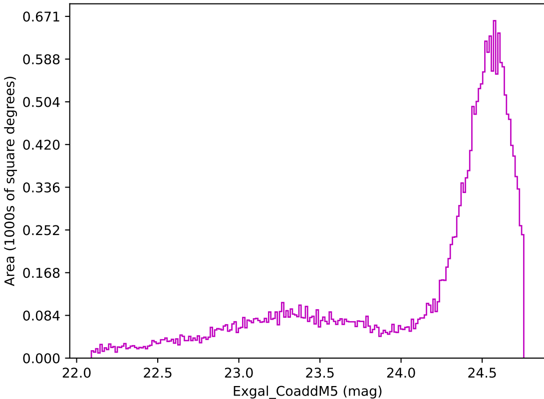
noroll_v3.4_10yrs Yr 1 z band: Exgal_CoaddM5
