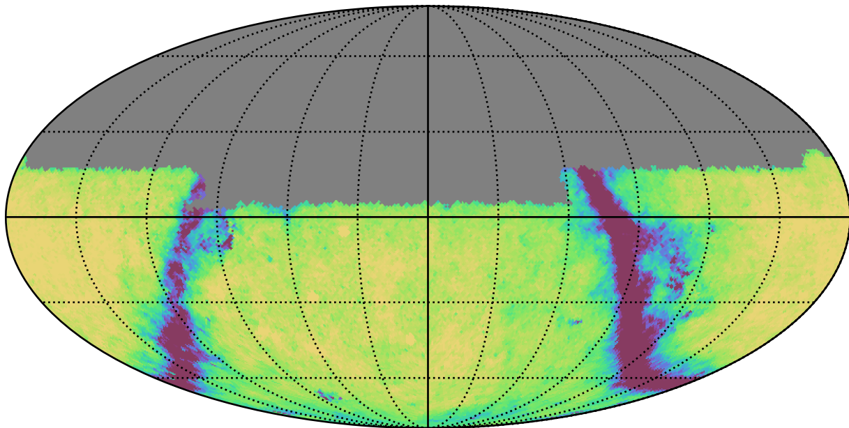
noroll_v3.4_10yrs Yr 1 u band: Exgal_CoaddM5
