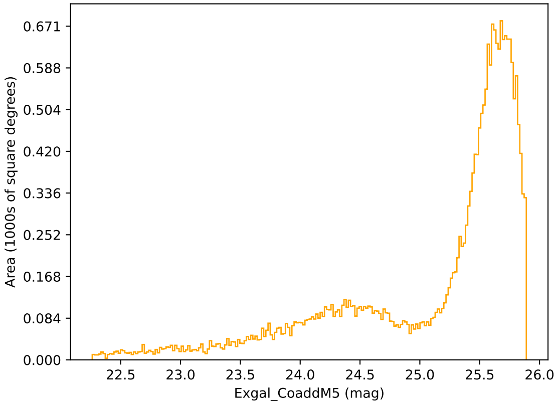
noroll_v3.4_10yrs Yr 1 r band: Exgal_CoaddM5
