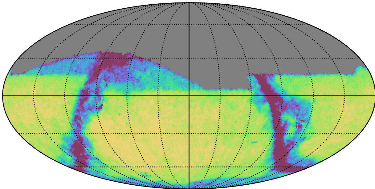
noroll_v3.4_10yrs Yr 1 i band: Exgal_CoaddM5
