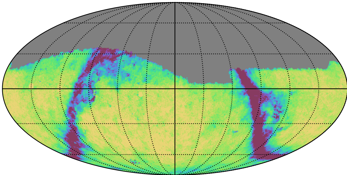
noroll_v3.4_10yrs Yr 1 g band: Exgal_CoaddM5
