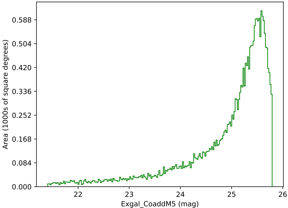
noroll_v3.4_10yrs Yr 1 g band: Exgal_CoaddM5
