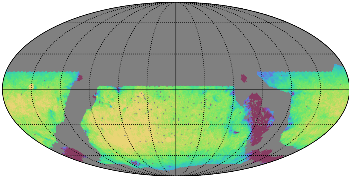
noroll_v3.4_10yrs WFD z band: Exgal_CoaddM5
