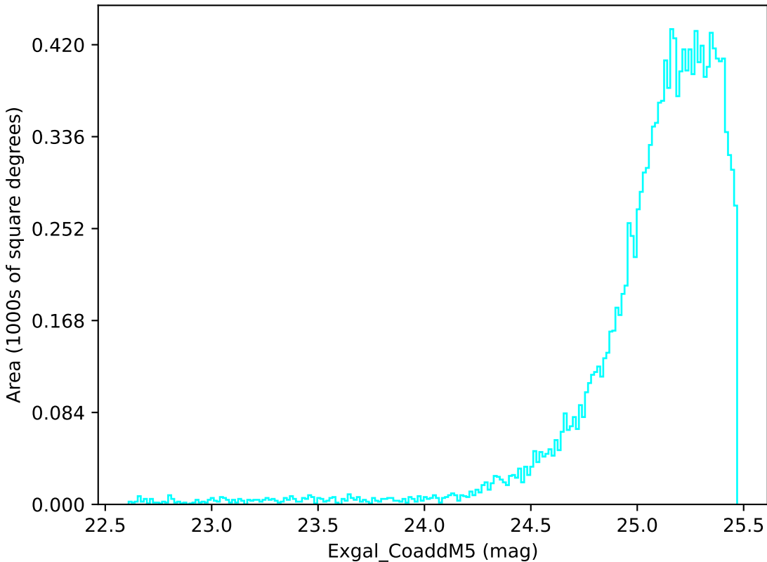
noroll_v3.4_10yrs WFD u band: Exgal_CoaddM5
