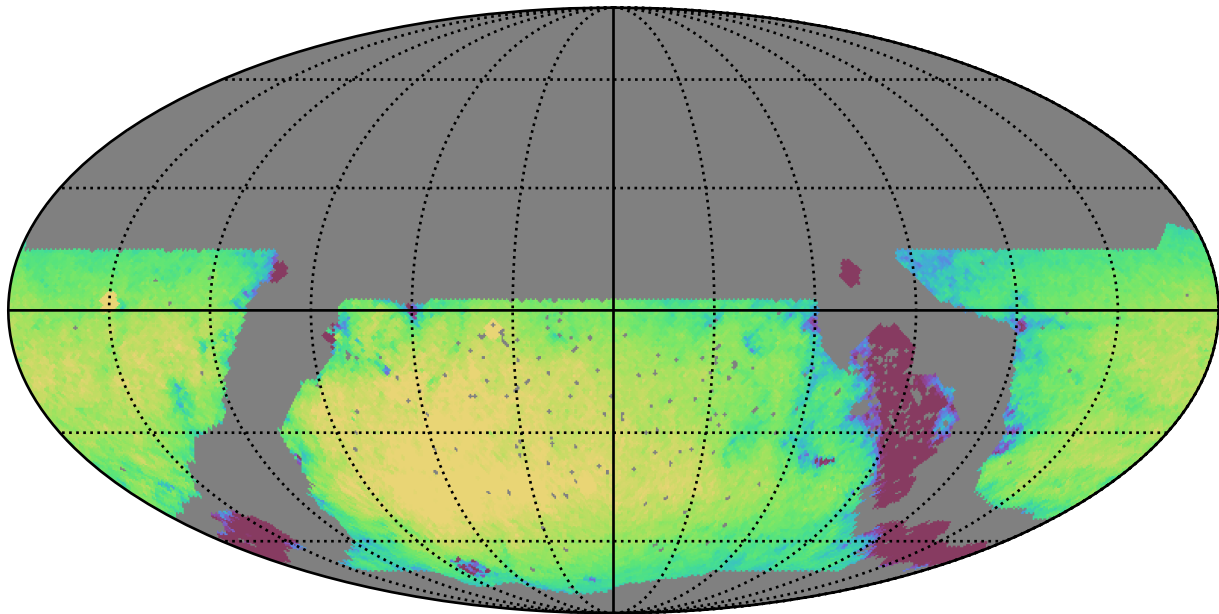
noroll_v3.4_10yrs WFD r band: Exgal_CoaddM5
