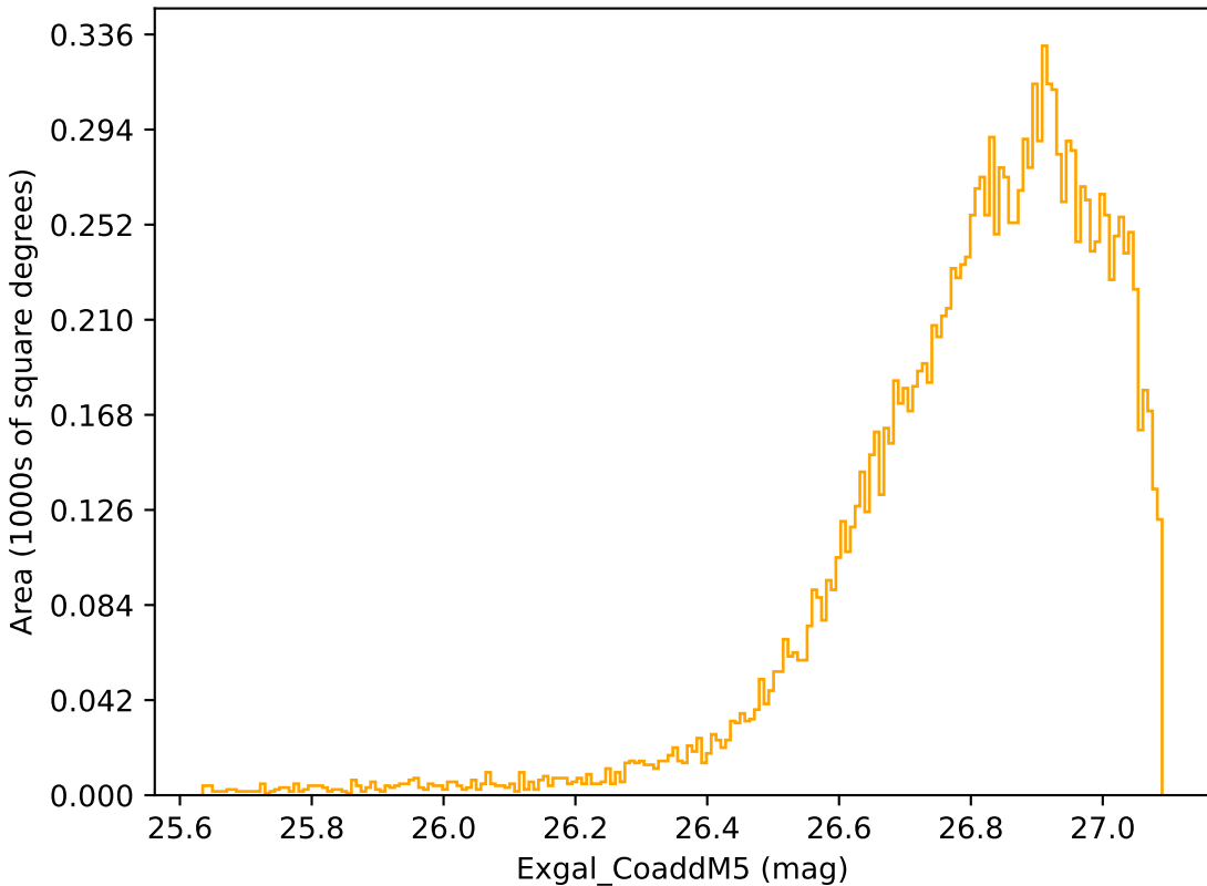
noroll_v3.4_10yrs WFD r band: Exgal_CoaddM5
