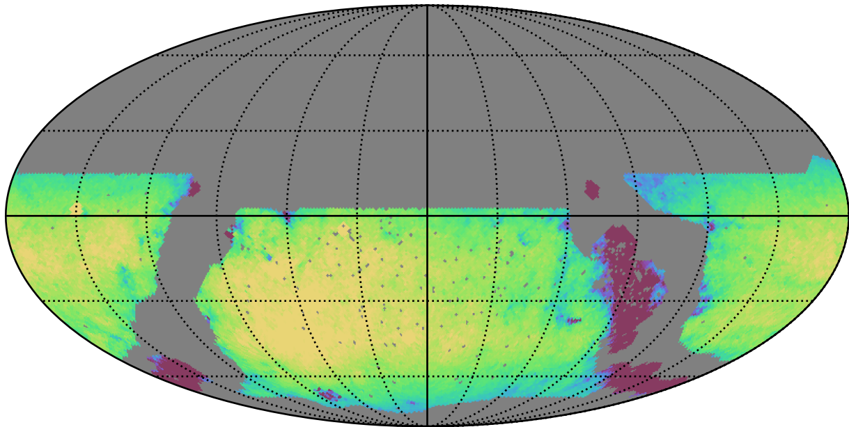
noroll_v3.4_10yrs WFD i band: Exgal_CoaddM5
