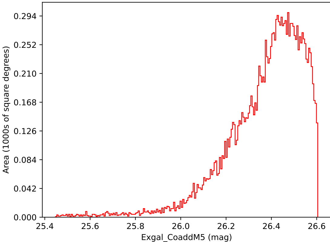
noroll_v3.4_10yrs WFD i band: Exgal_CoaddM5
