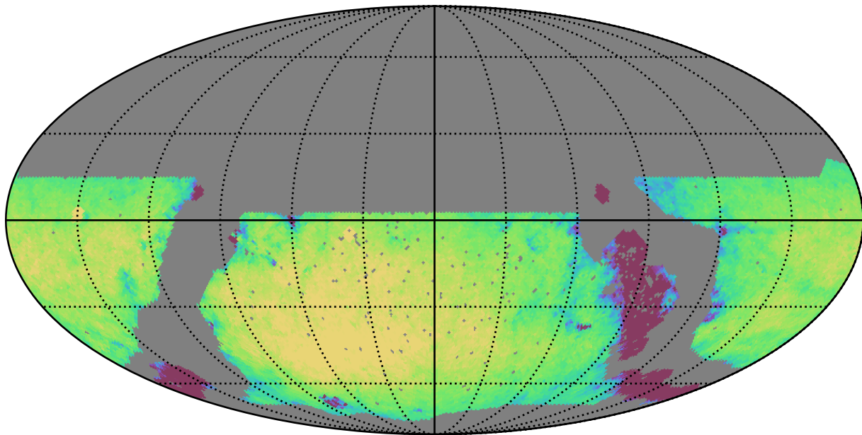
noroll_v3.4_10yrs WFD g band: Exgal_CoaddM5
