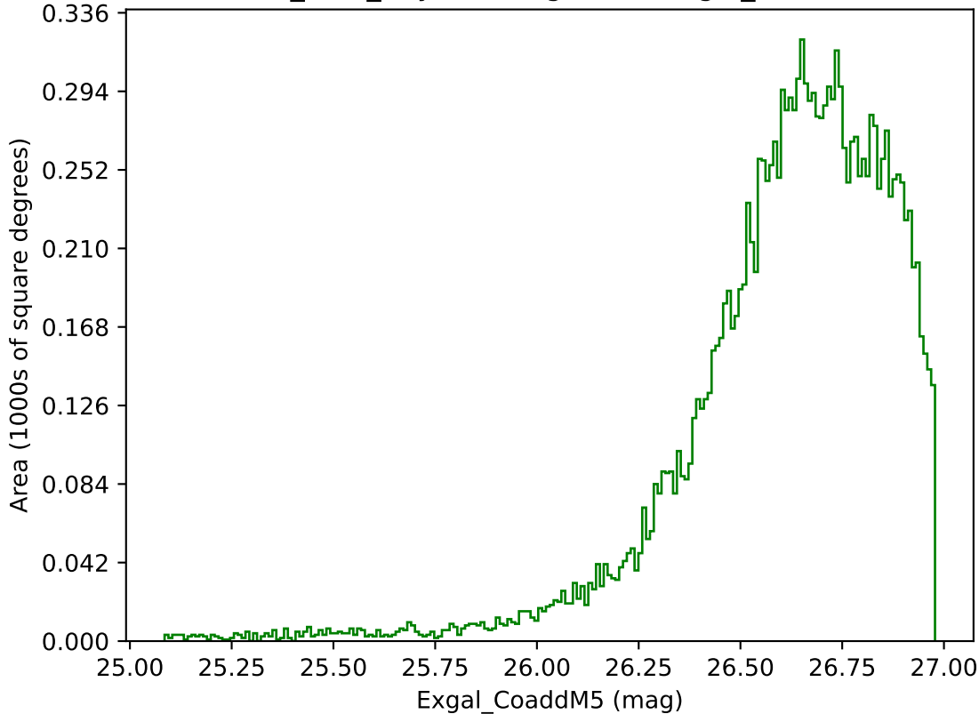
noroll_v3.4_10yrs WFD g band: Exgal_CoaddM5
