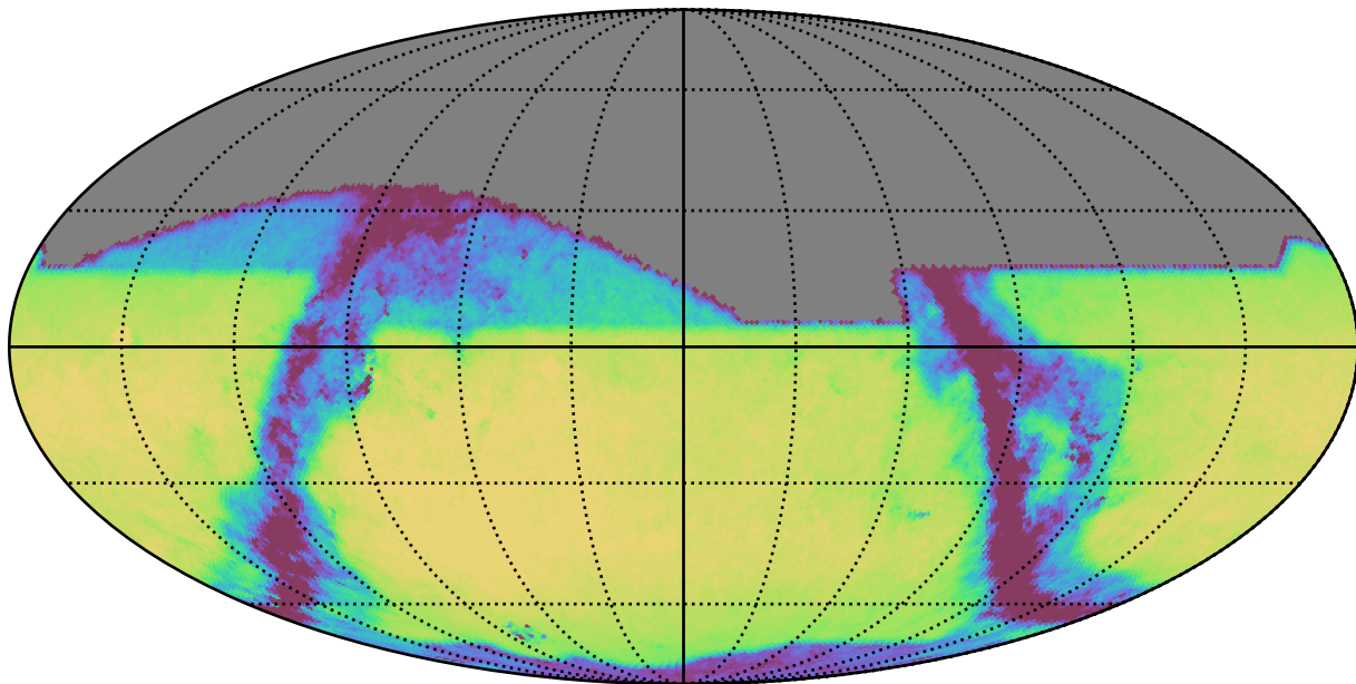
noroll_v3.4_10yrs All sky z band: Exgal_CoaddM5
