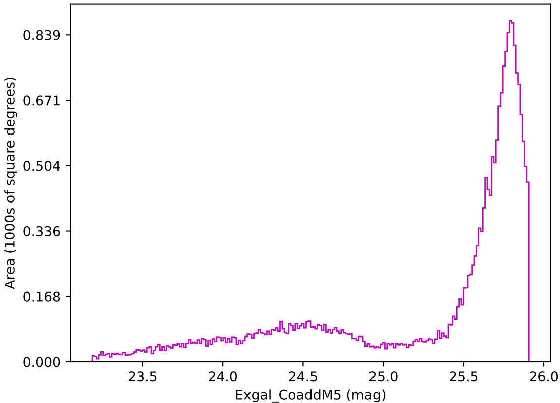
noroll_v3.4_10yrs All sky z band: Exgal_CoaddM5
