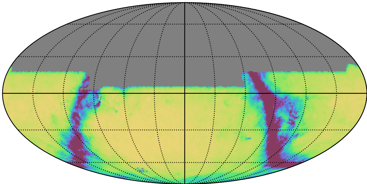
noroll_v3.4_10yrs All sky u band: Exgal_CoaddM5
