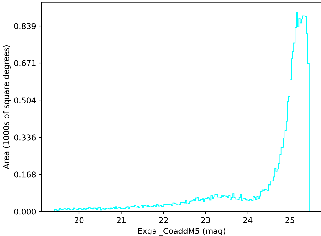
noroll_v3.4_10yrs All sky u band: Exgal_CoaddM5
