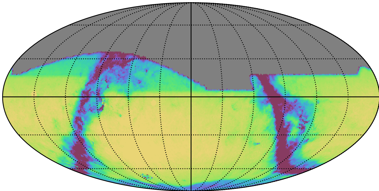
noroll_v3.4_10yrs All sky r band: Exgal_CoaddM5
