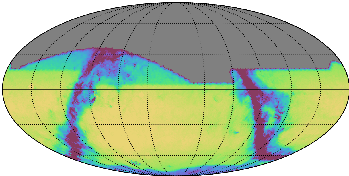
noroll_v3.4_10yrs All sky i band: Exgal_CoaddM5
