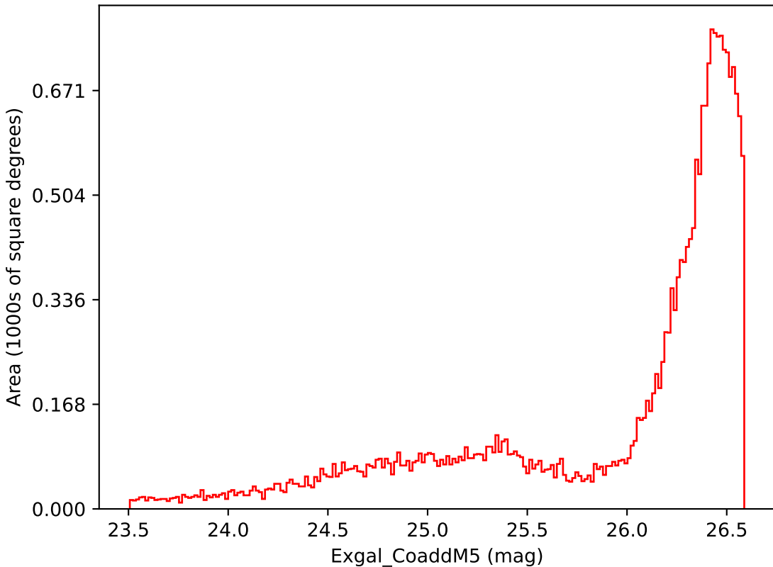
noroll_v3.4_10yrs All sky i band: Exgal_CoaddM5
