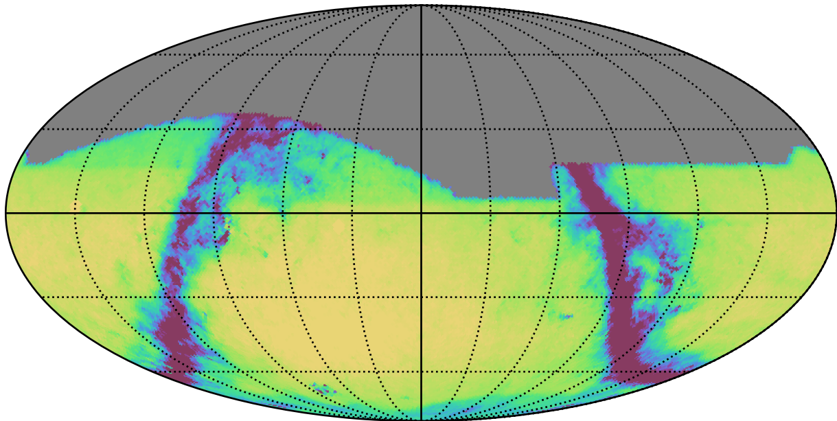
noroll_v3.4_10yrs All sky g band: Exgal_CoaddM5
