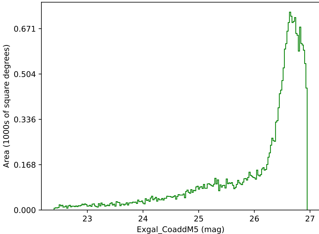
noroll_v3.4_10yrs All sky g band: Exgal_CoaddM5
