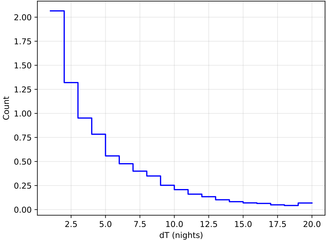
noroll_v3.4_10yrs WFD all bands: DeltaNight Histogram
