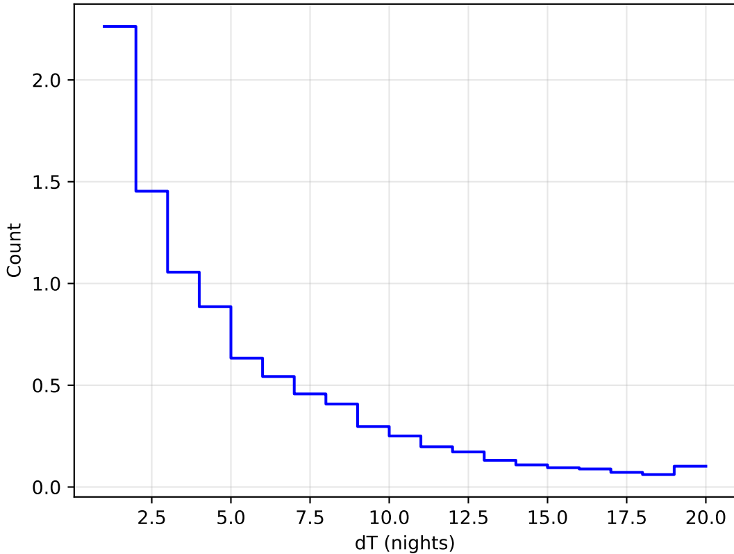
noroll_v3.4_10yrs All sky all bands: DeltaNight Histogram 1e6
