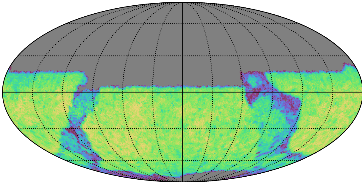
noroll_v3.4_10yrs Yr 3-4 y band: CoaddM5
