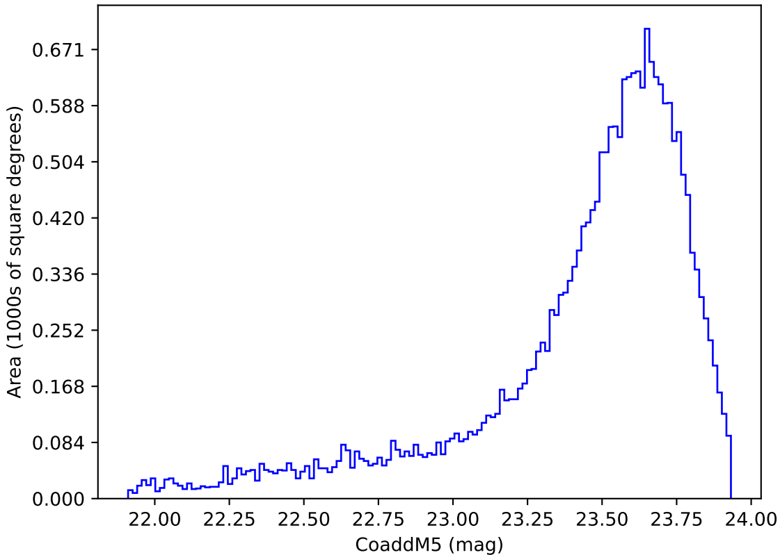
noroll_v3.4_10yrs Yr 3-4 y band: CoaddM5
