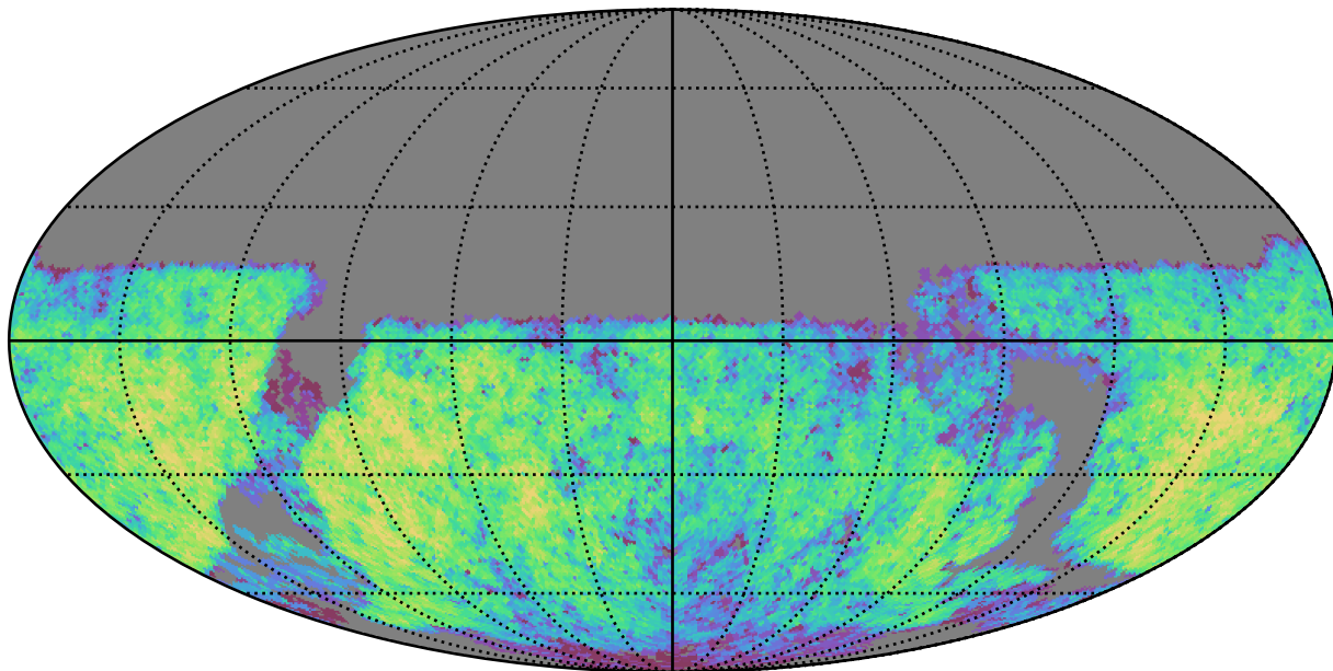
noroll_v3.4_10yrs Yr 3-4 u band: CoaddM5
