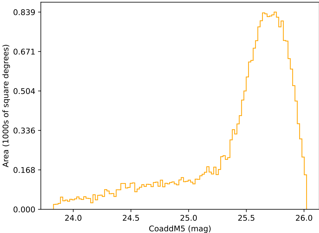
noroll_v3.4_10yrs Yr 3-4 r band: CoaddM5
