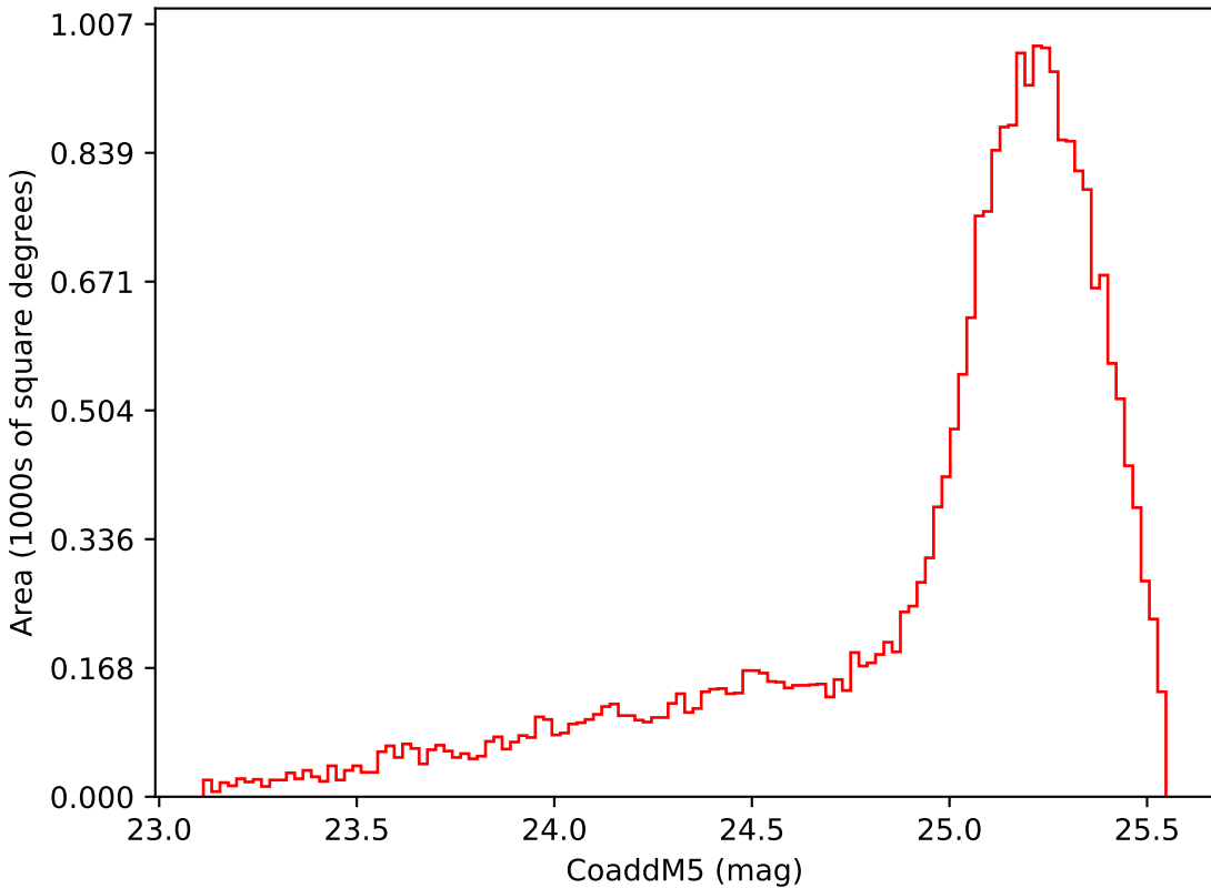
noroll_v3.4_10yrs Yr 3-4 i band: CoaddM5
