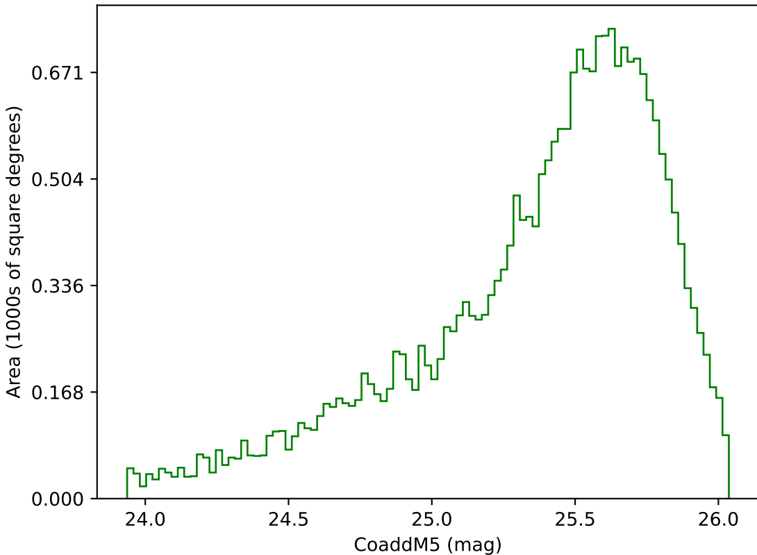
noroll_v3.4_10yrs Yr 3-4 g band: CoaddM5
