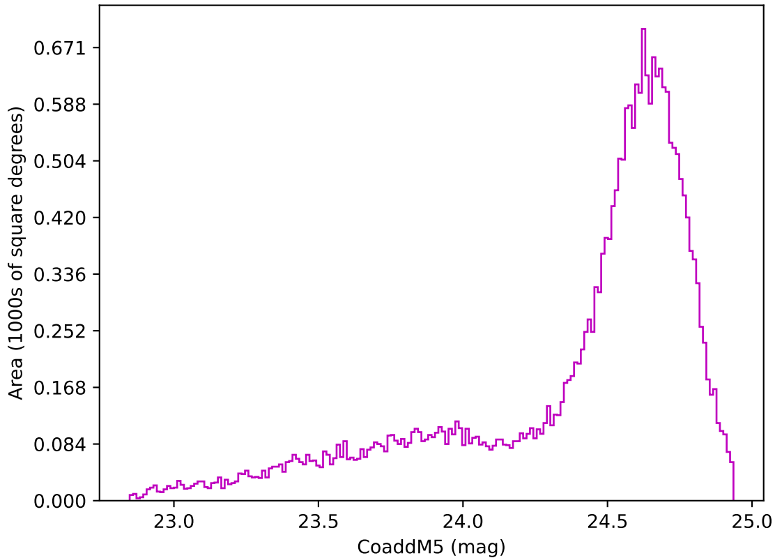
noroll_v3.4_10yrs Yr 1 z band: CoaddM5
