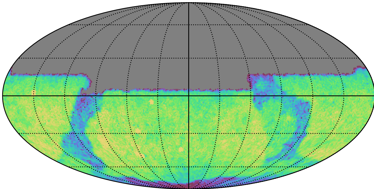
noroll_v3.4_10yrs Yr1 y band: CoaddM5
