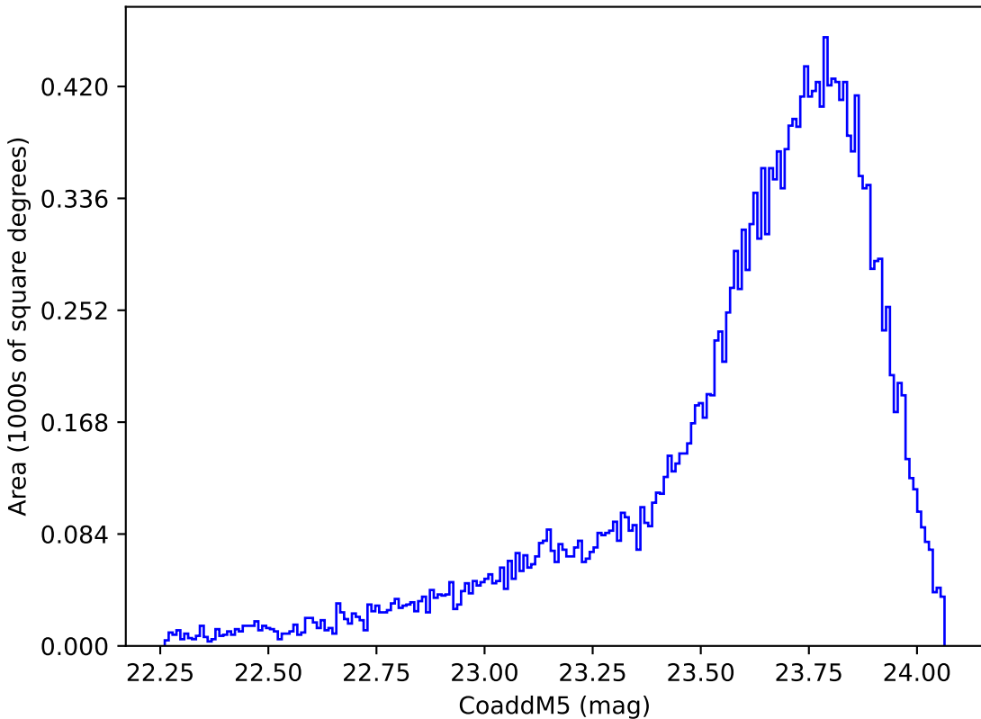
noroll_v3.4_10yrs Yr 1 y band: CoaddM5
