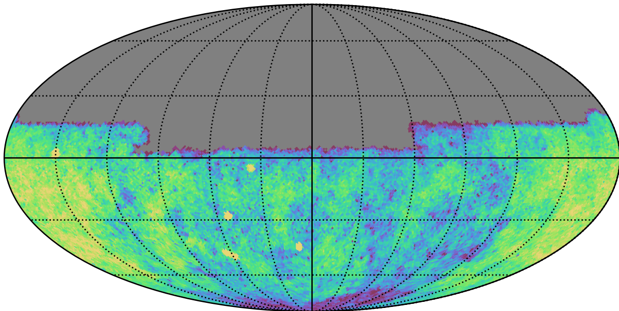
noroll_v3.4_10yrs Yr 1 u band: CoaddM5
