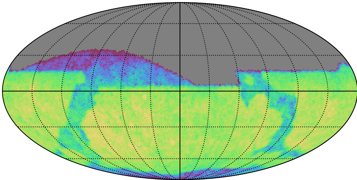
noroll_v3.4_10yrs Yr 1 i band: CoaddM5
