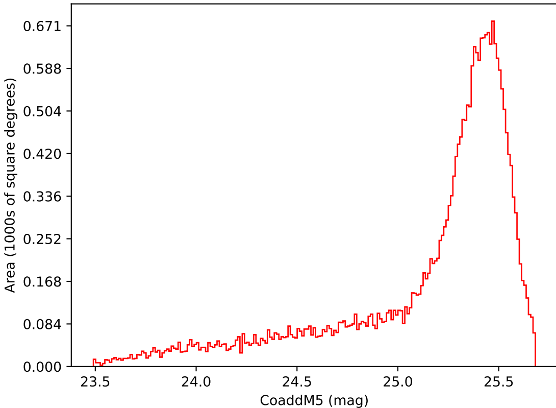
noroll_v3.4_10yrs Yr 1 i band: CoaddM5
