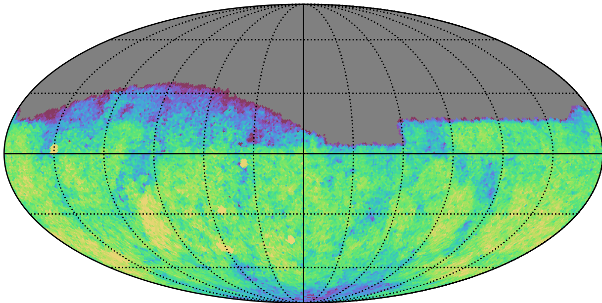
noroll_v3.4_10yrs Yr 1 g band: CoaddM5
