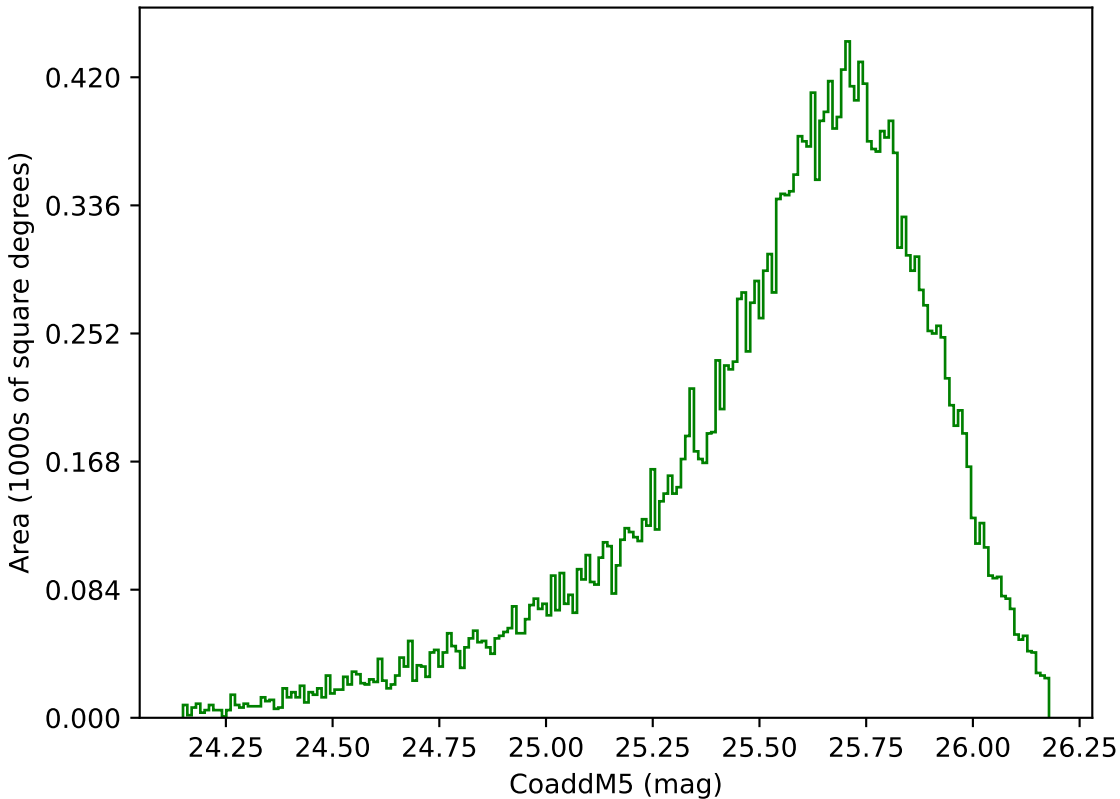
noroll_v3.4_10yrs Yr 1 g band: CoaddM5
